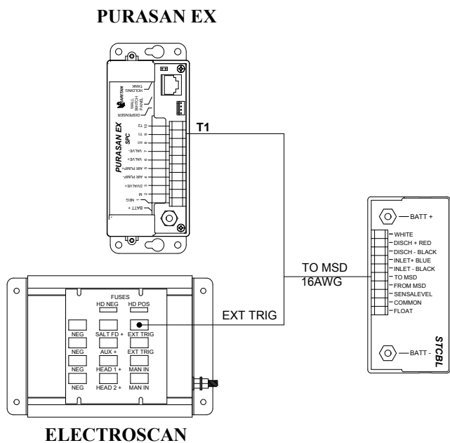
FIG 6 WIRING FOR SMART TOILET CONTROL WITH MSD PURASAN EX
